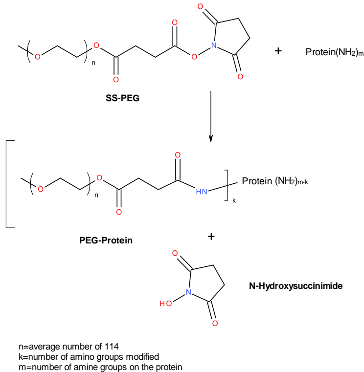
Figure 2: Reaction between SS-PEG and a Protein
